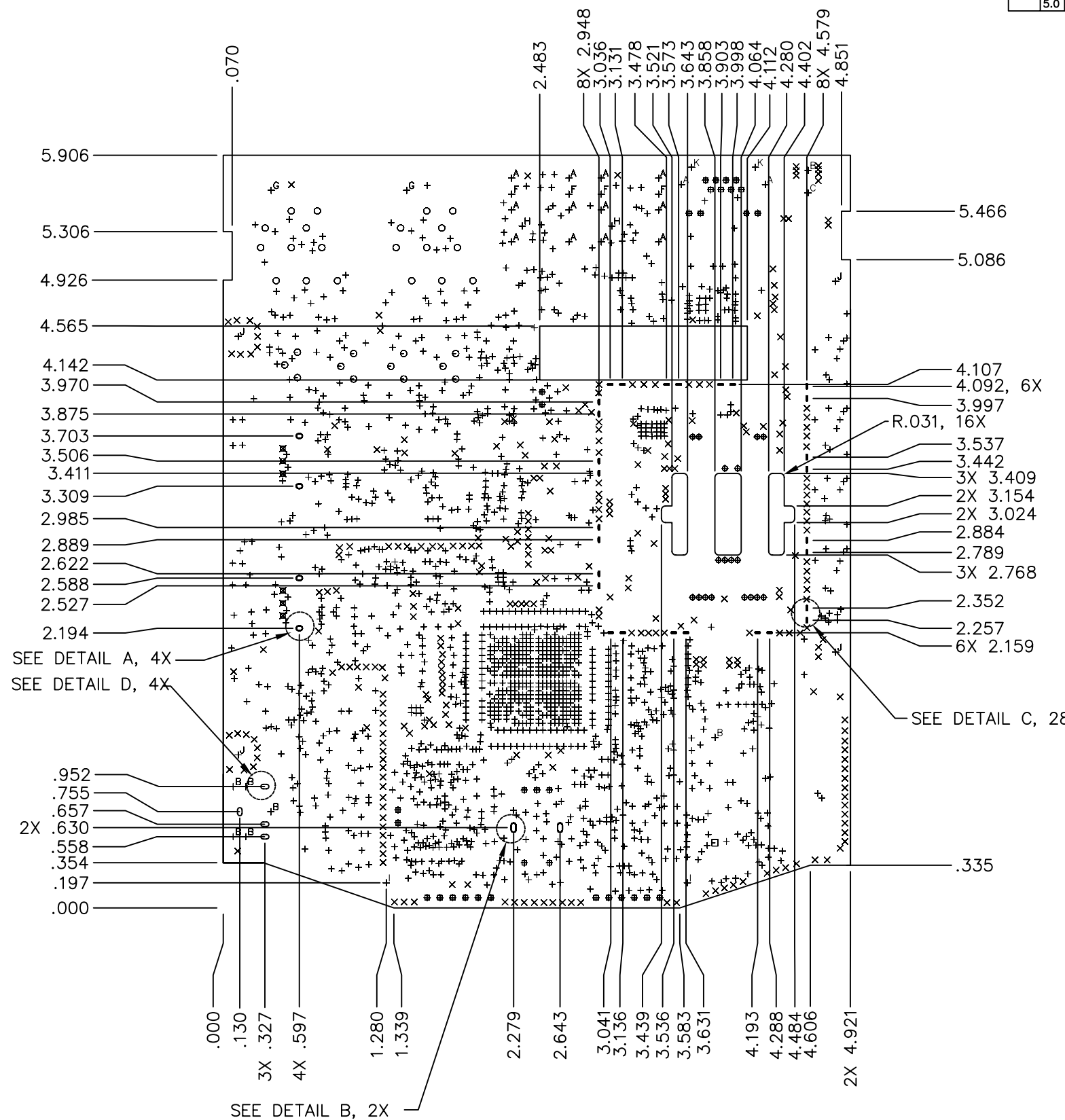
DRILL AND TRIM VIEW
