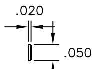
DETAIL C (PLATED)
