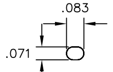
DETAIL A (PLATED)
