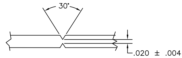
DETAIL A FINAL EDGE OF PC BOARD
